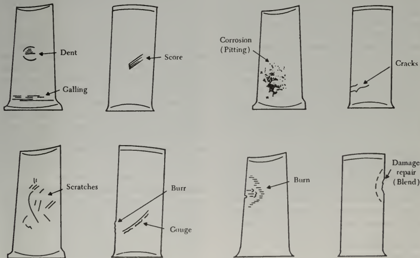
FIGURE 10-56. Compressor blade damage.
